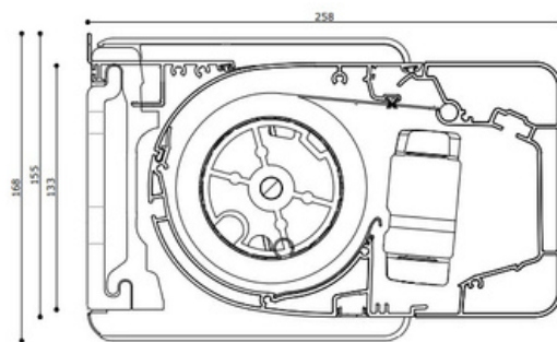
Wandmontage
